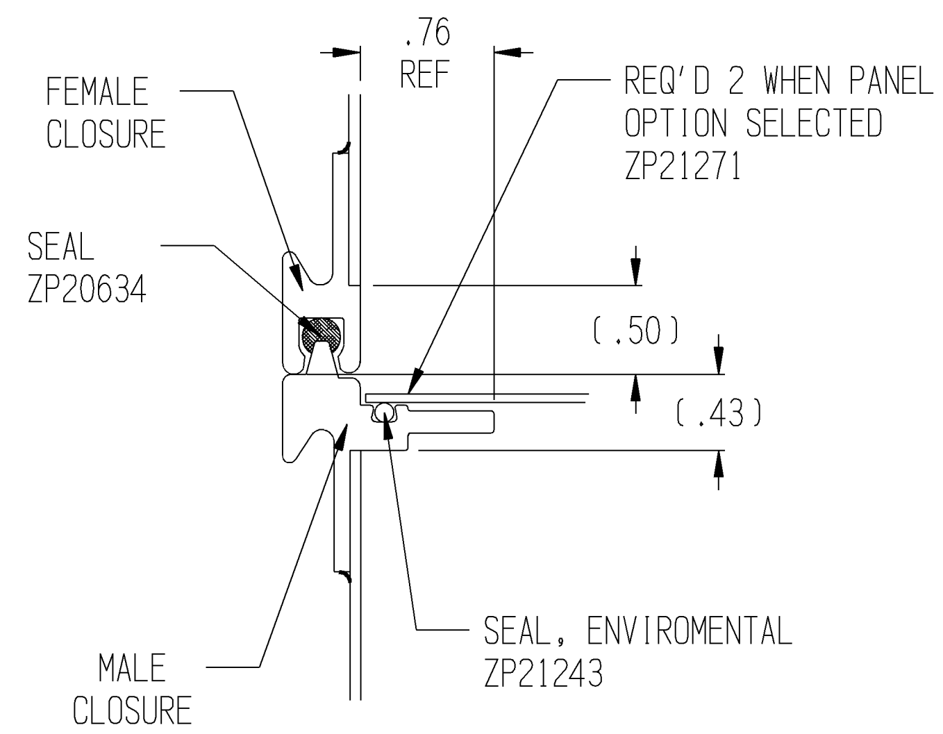
CLOSURE DETAIL FOR WATERTIGHT, DRIP PROOF AND MIL-T-28800 STYLE A
