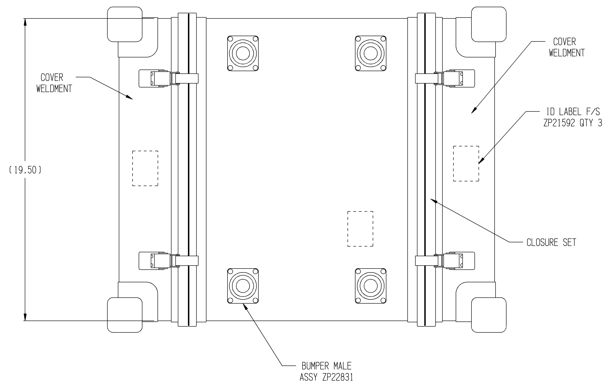
VIEW FOR MIL-T-28800 STYLE "A" OPTION
