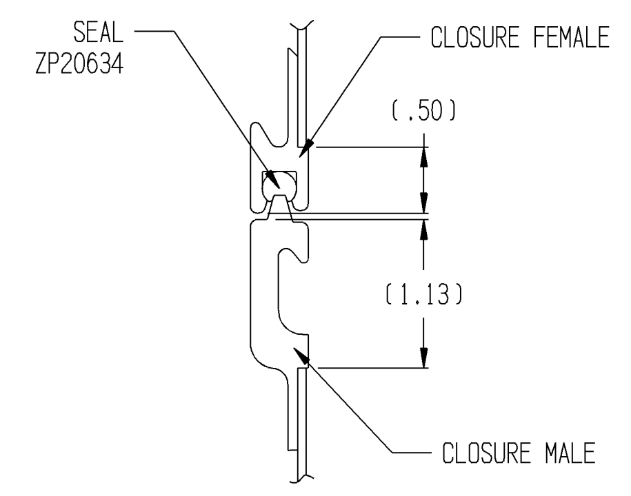
CLOSURE DETAIL SCALE 1:1
